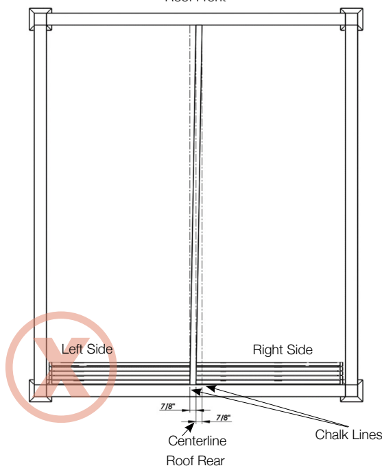
Misaligned Drive Beam
