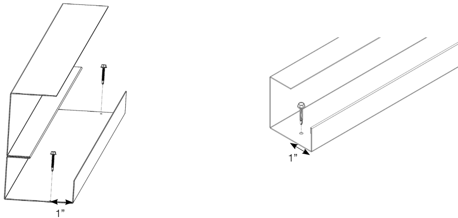
Vertical Attachment of the Stabilizers
